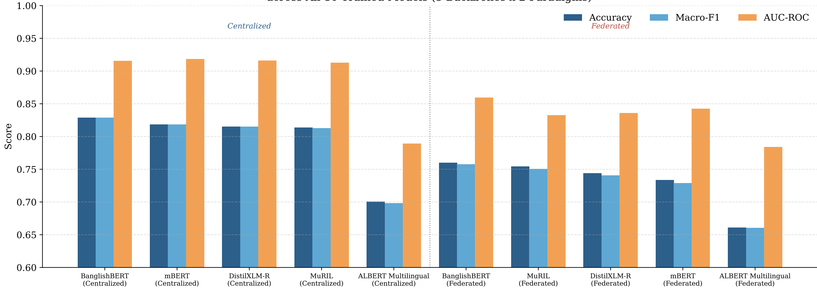
Overall Performance Comparison: Accuracy, Macro-F1, and AUC-ROC across All 10 Trained Models (5 Backbones x 2 Paradigms)
